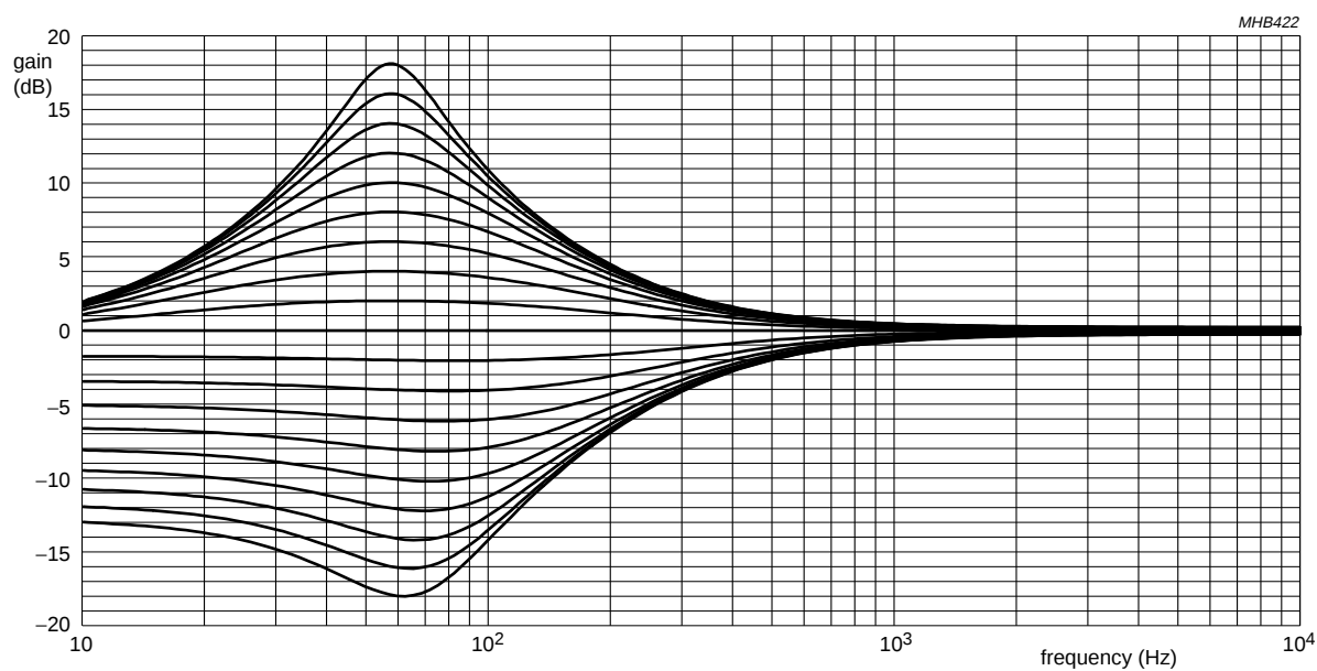
Fig.17 Bass curve with 2 \times 220 nF and R = 3.3 k \Omega external, BSYB = 1 for gain and BSYC = 0 for cut.
